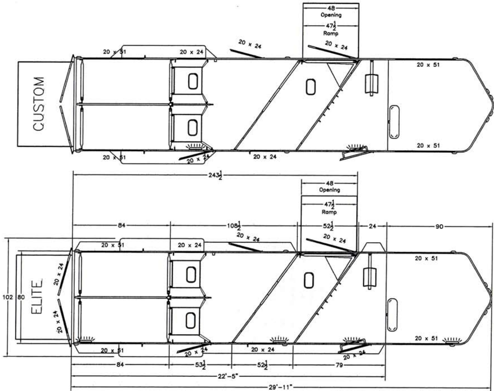
3 HORSE GOOSENECK WALK-THRU SLANT W/DRESS
